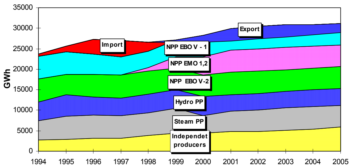
Fig. 5. Development of Electricity Generation
