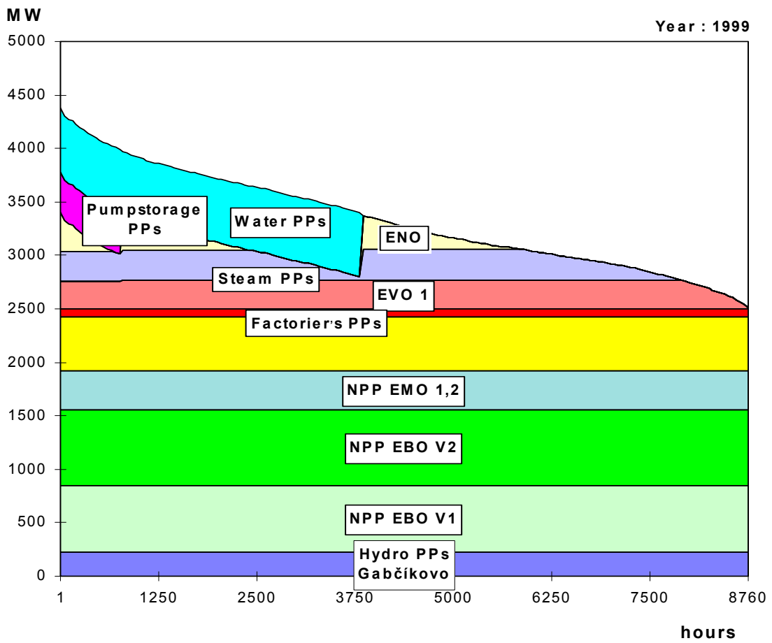
Fig. 7. Annual Load Follow Curve of the Slovak Electricity System
